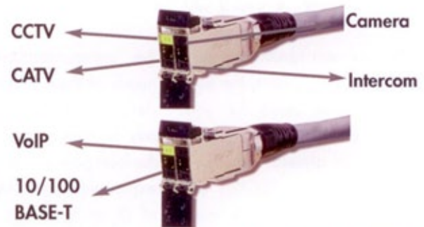
Figure 1: Typical Multi-Application Cable Sharing Implementation
